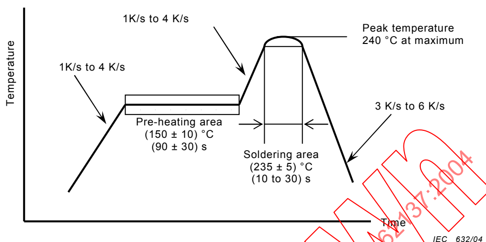
Figure 3 – Reflow profile
