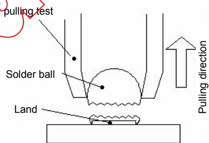
Figure A.3b – Ball pinch method
