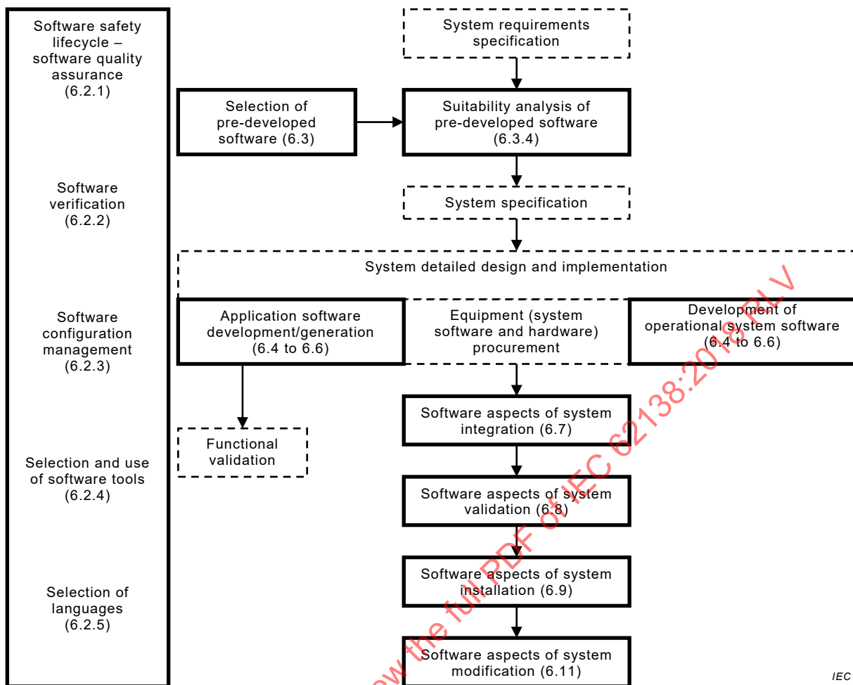
Figure 3 – Software related activities in the system safety lifecycle
