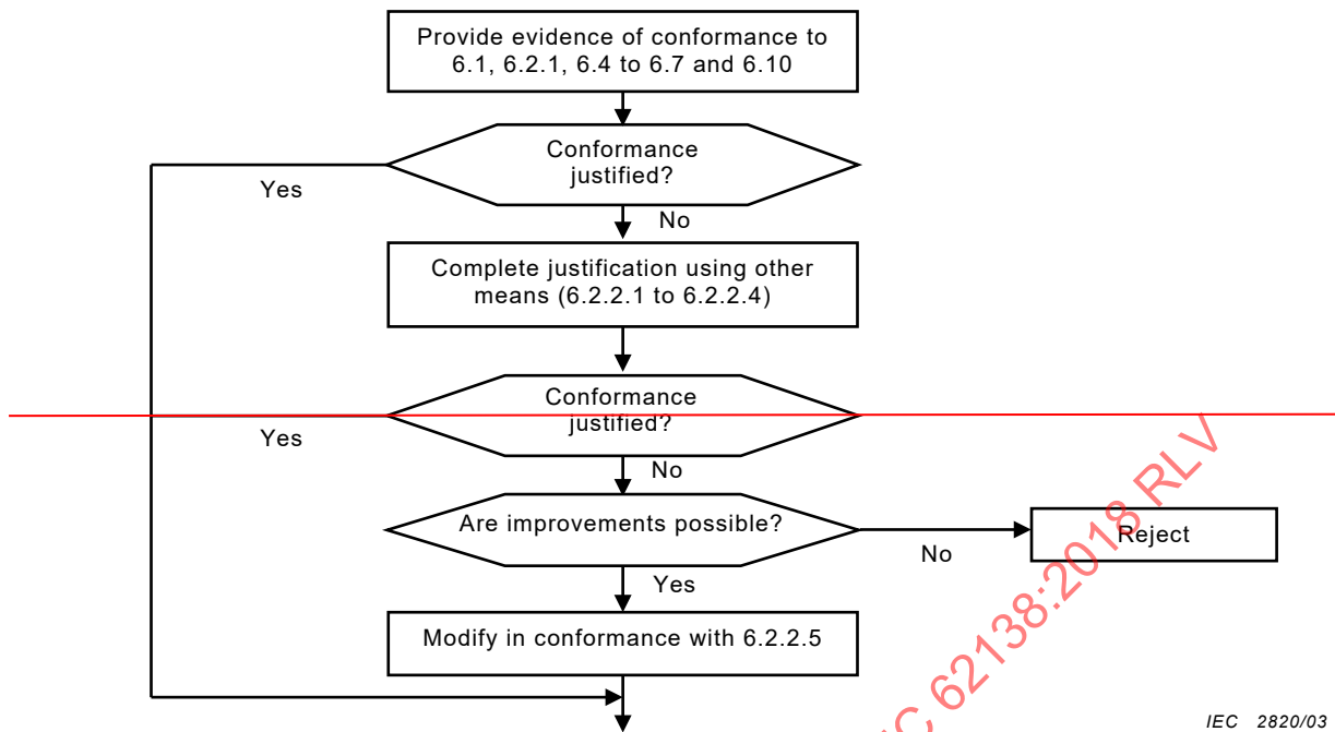
Figure 5 — Process for providing evidence of correctness for pre-developed software of an I&C system of safety class 2
