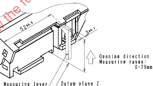
Figure 22 – Lid unlocking force (L-cassette)
