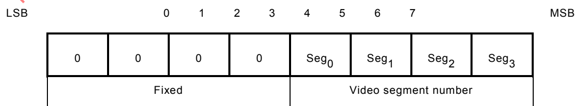
Figure 52 – Macro block identifier byte descriptions
