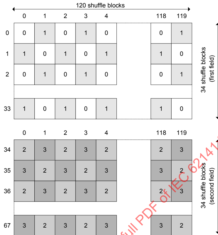
Figure 41 – 1920 × 1080/I 4:2:2 YC B C R shuffle sets
