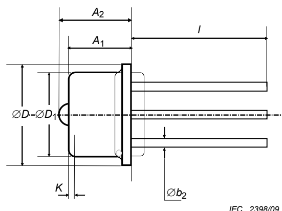
b) Outside drawing of TO CAN with a ball lens
