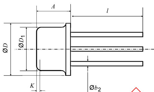
Figure 4a – Outside drawing of TO CAN with flat window
