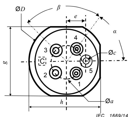
Figure 7 – Schematic diagram of VCSEL TOSA package with LC connector and with optional colour code C for pin-type notation for use at high speed (≥8 Gbps)
