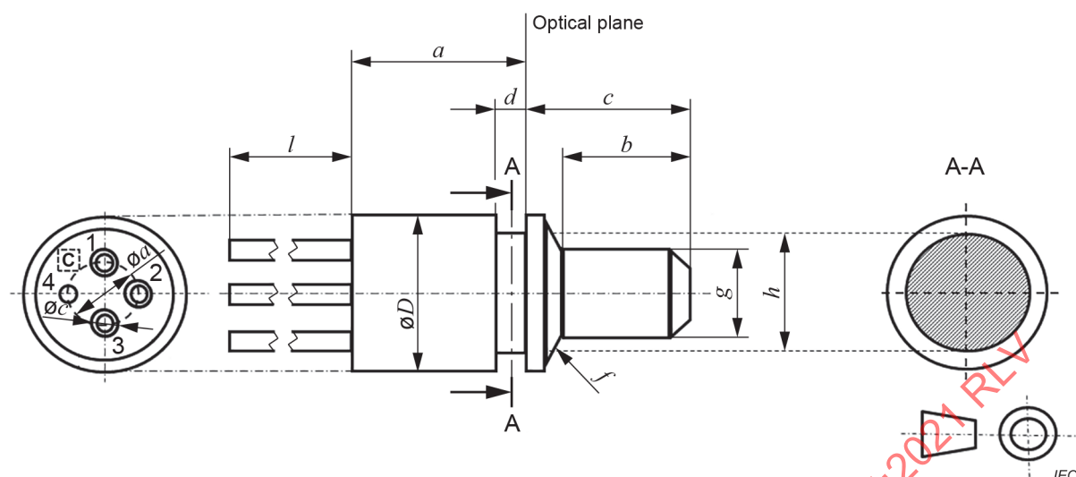
Figure 6 – Schematic diagram of VCSEL TOSA package with SC connector and with optional colour code C on the bottom for uses at low speed (below 8 Gbps Gbit/s)
