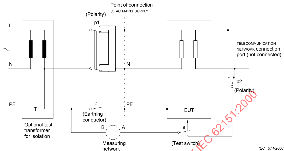
Figure 5 – Test circuit for touch current of single-phase equipment on a star TN or TT power supply system
