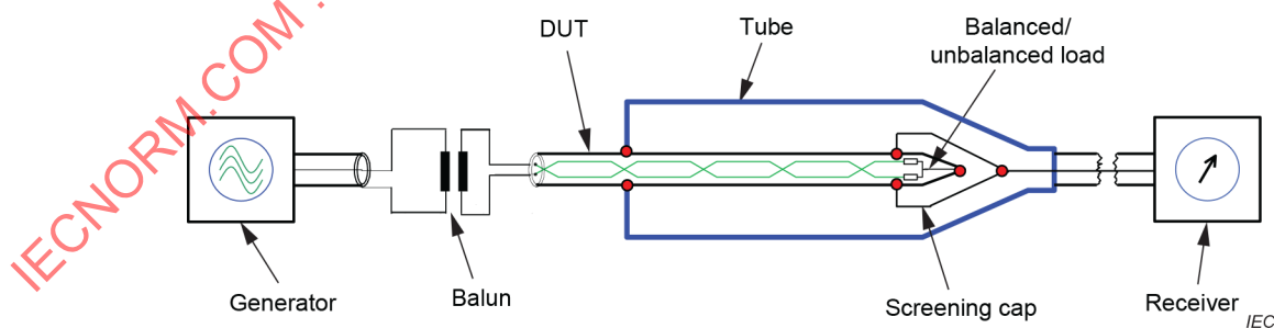
Figure A.3 – Coupling attenuation, principle of test setup with balun and standard tube
