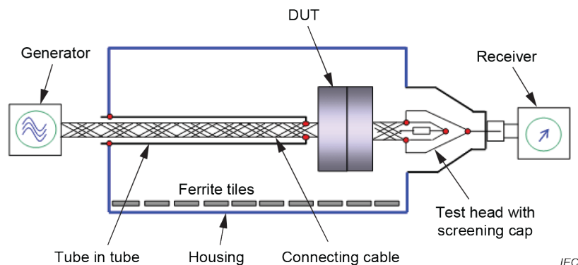
Figure C.3 – Principle of the triaxial cell with tube in tube and ferrite tiles as absorber
