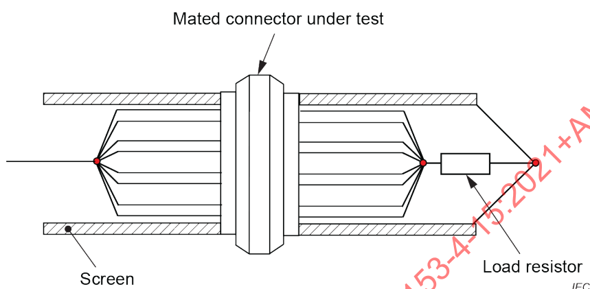
Figure 5 – Preparation of balanced or multipin connectors for transfer impedance and screening attenuation
