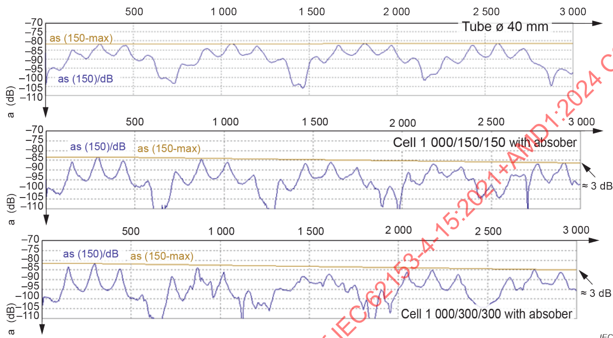
Figure C.4 – Comparison of the measurements of an RG 214 with 40 mm tube and triaxial cells with magnetic absorber
