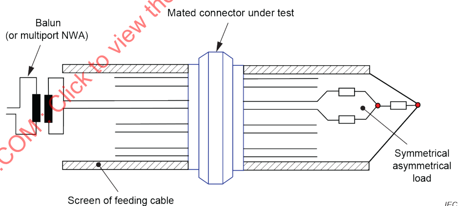
Figure 6 – Preparation of balanced or multipin connectors for coupling attenuation measurement
