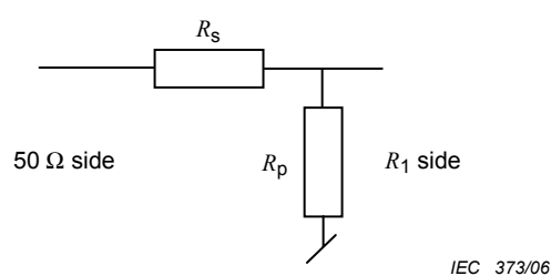
Figure 7 – Impedance matching for Z_1 < 50 \Omega
