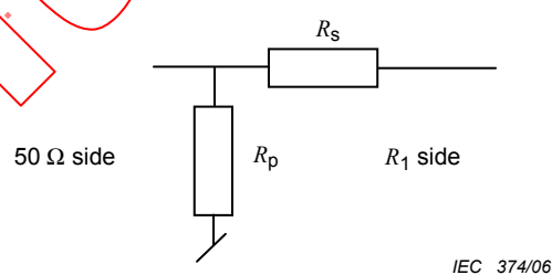
Figure 8 – Impedance matching for Z_1 > 50 \Omega
