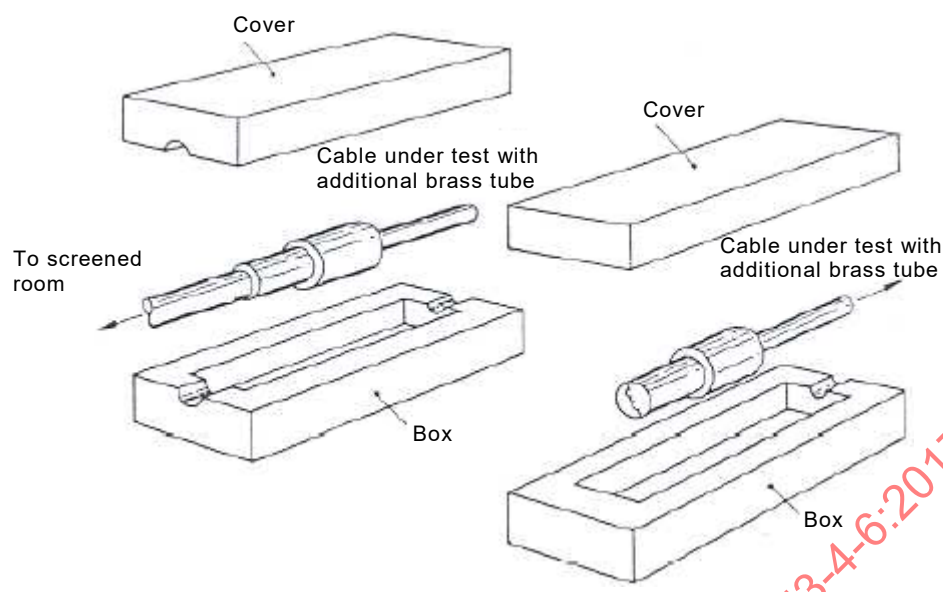
Figure 8 – Additional screening of connectors on the cable under test (CUT)
