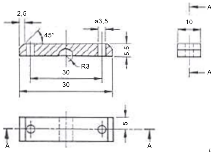
Figure 5 – Impedance matching part of launcher injection feature – Position 3
