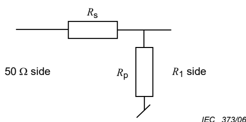
Figure 7 — Impedance matching for Z_1 < 50 \Omega
