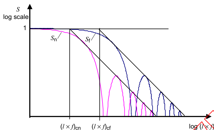
Figure A.2 – Summing function S
