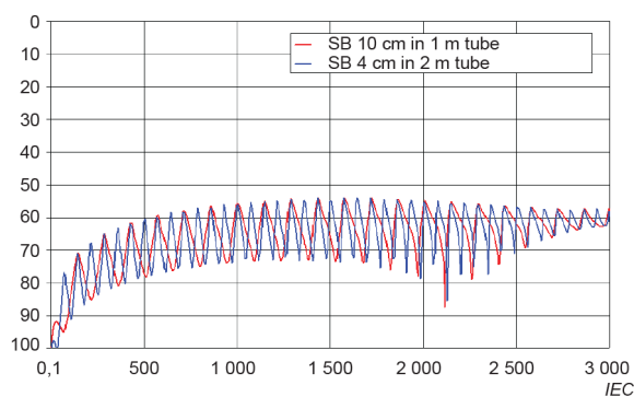
Figure C.14 – simulation, linear frequency scale
