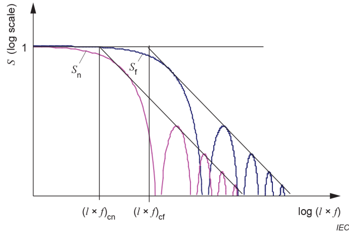
Figure C.2 – Summing function S
