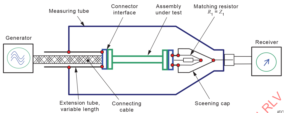
Figure E.2 – Principle of the test set-up to measure transfer impedance and screening attenuation of a cable assembly
