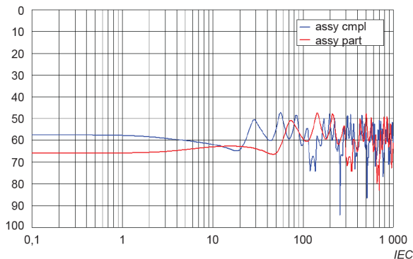
Figure C.5 – Simulation of a cable assembly (logarithmic scale)
