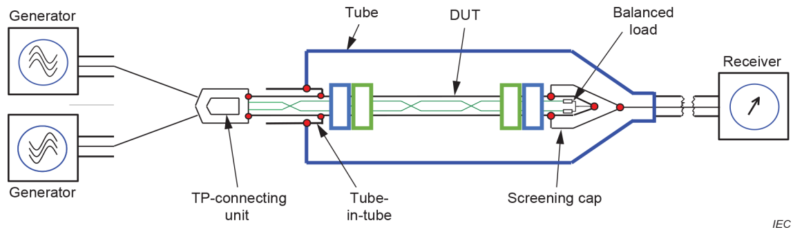
Figure 10 – Coupling attenuation, principle test set-up with multiport VNA and TP-connecting unit for measuring complete cable assemblies
