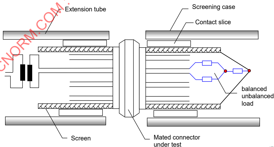
c) Principle preparation of balanced or multiconductor connectors for coupling attenuation using a balun
