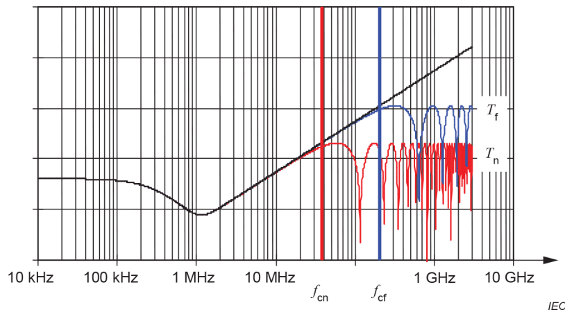
Figure C.3 – Calculated coupling transfer function ( l = 1 m; \epsilon_{r1} = 2,3 ; \epsilon_{r2} = 1 ; Z_F = 0 )
