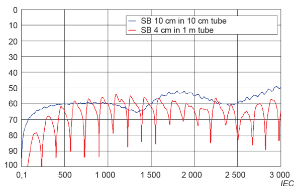
Figure C.12 – Measurement, linear frequency scale
