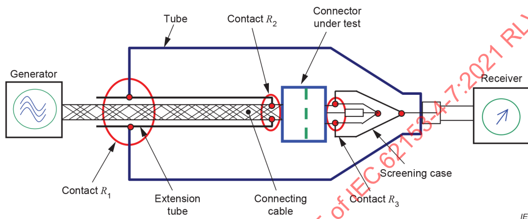
Figure D.1 – Contact resistances of the test set-up
