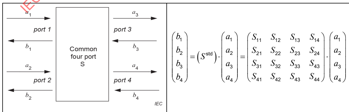
Figure F.2 – Common four port network
