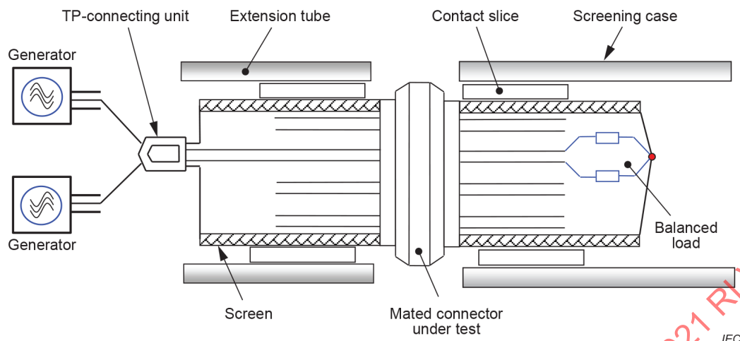
d) Principle preparation of balanced or multiconductor connectors for coupling attenuation using a virtual balun
