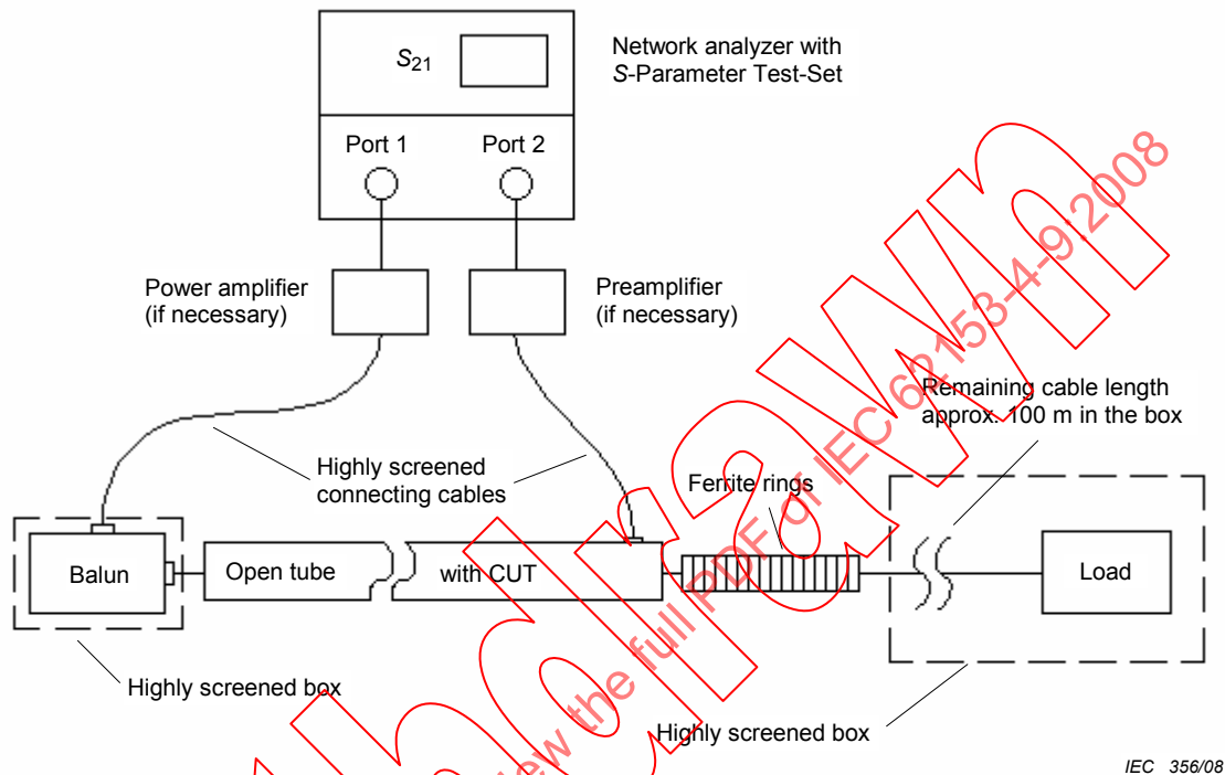
Figure 2 – Set-up to measure the coupling attenuation
