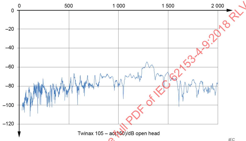
Figure 8 – Coupling attenuation Twinax 105, open head procedure
