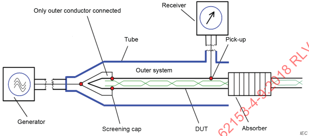
Figure 7 – Test set-up to measure a_{\text{tube}}
