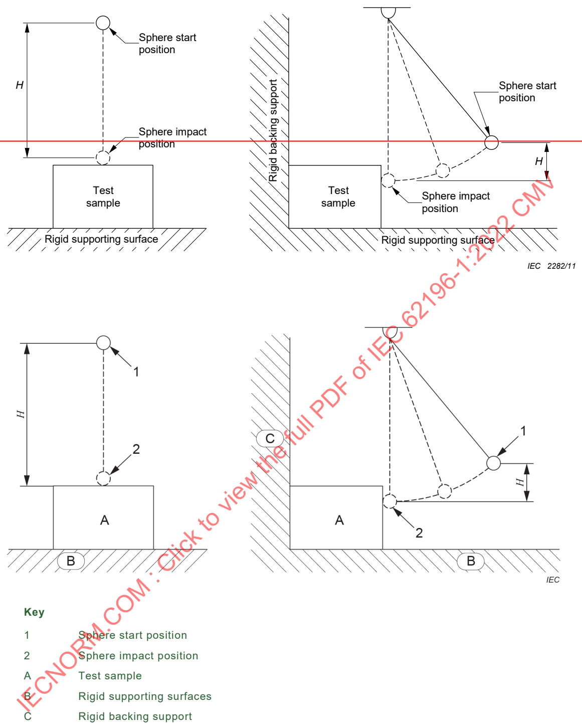
Figure 18 – Ball impact test
