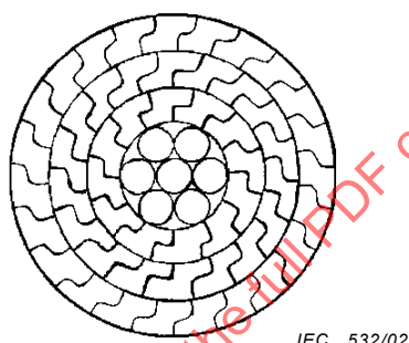
Figure 1b – Three-layer conductor made of formed wires type AxF/Sxy
