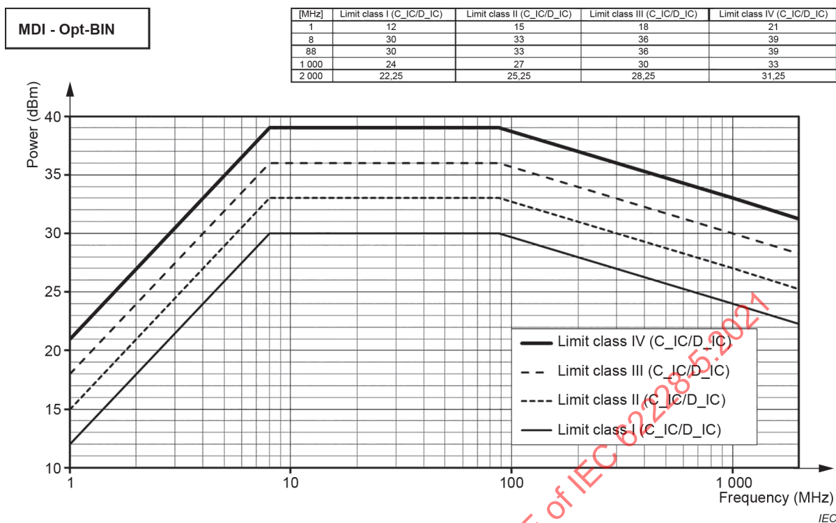
Figure D.5 – Example of limits for conducted RF immunity for functional status class C IC or D IC – MDI Opt-BIN
