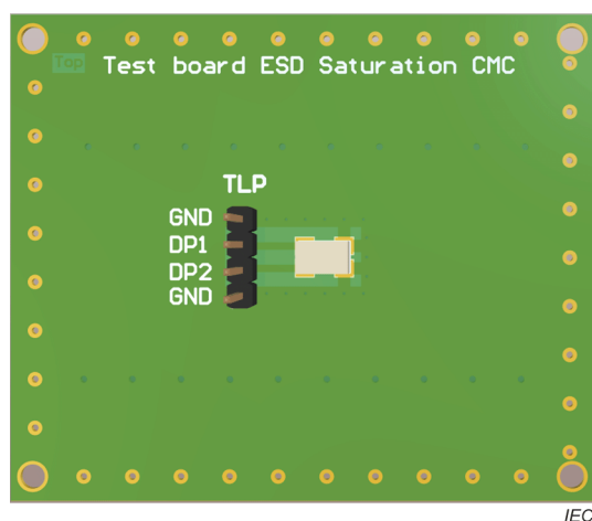
Figure E.15 – Example of ESD saturation test board for CMC, top layer
