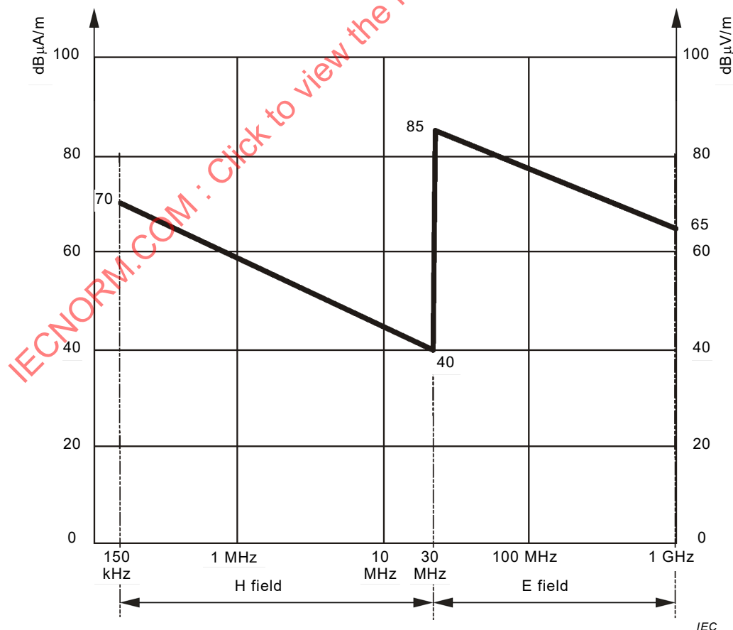
Figure A.1 – Emission from switches – Peak
