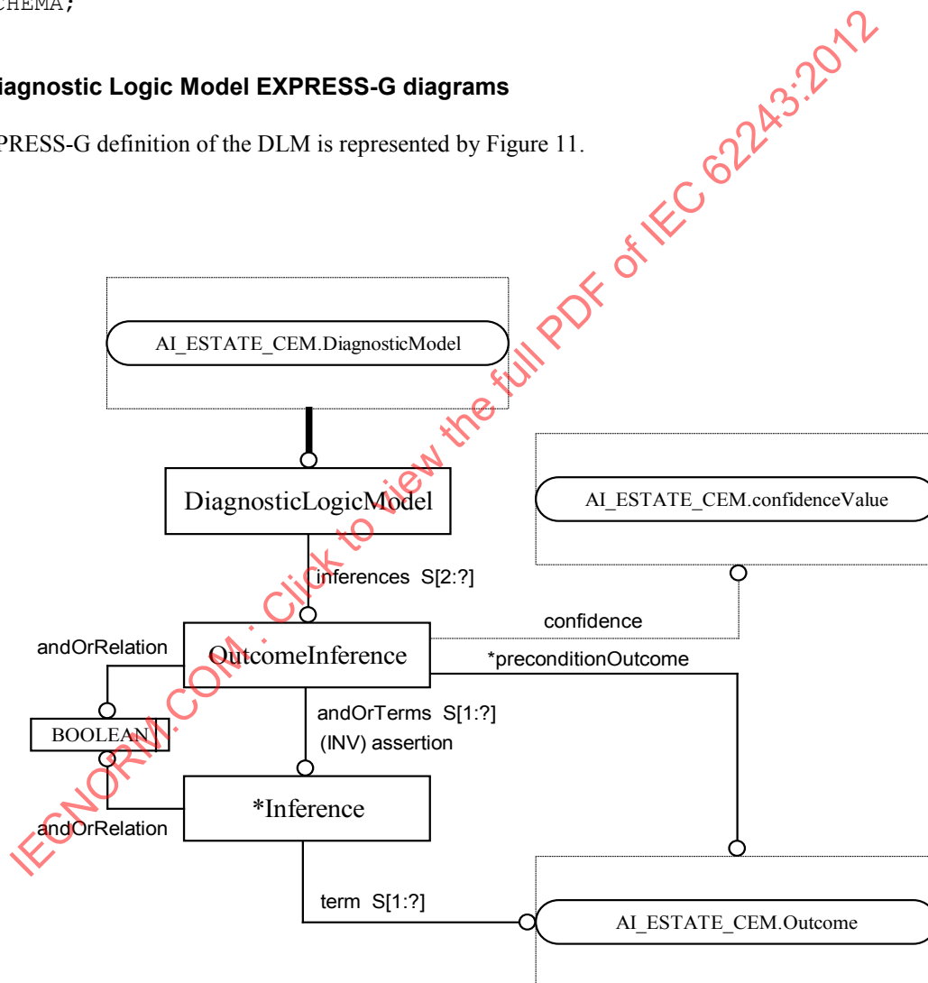
Figure 11 —AI_ESTATE_DLM EXPRESS-G diagram 1 of 1
