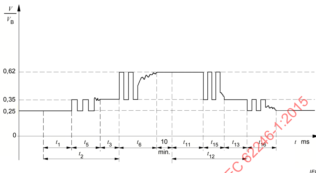
a) Break-before-make
