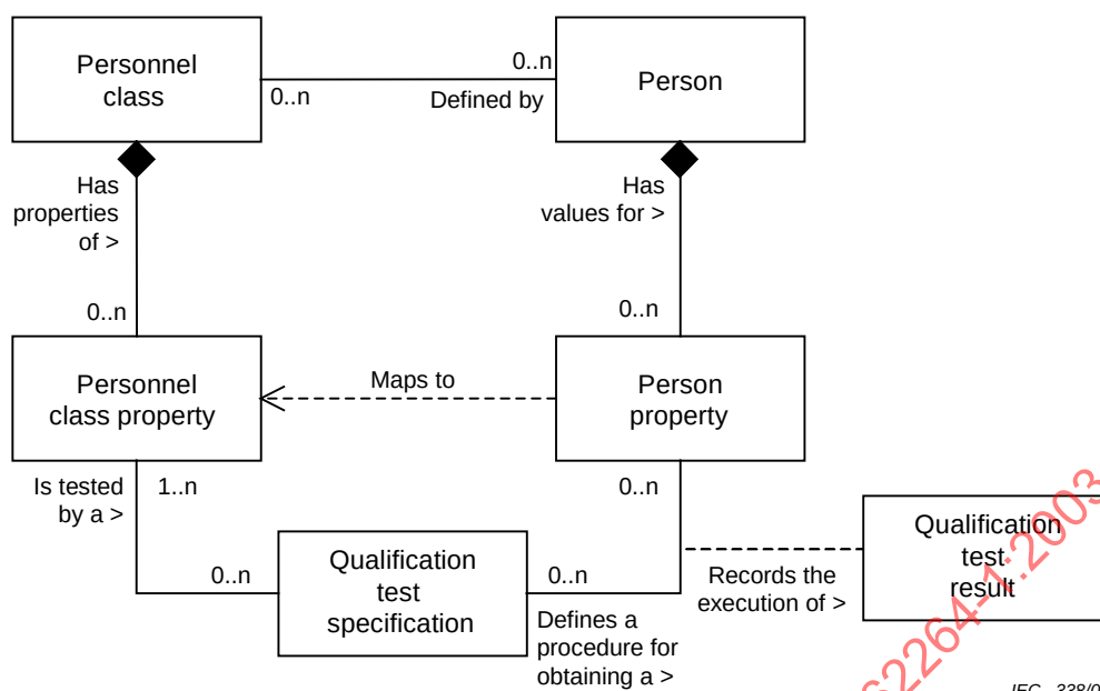
Figure 14 – Personnel model
