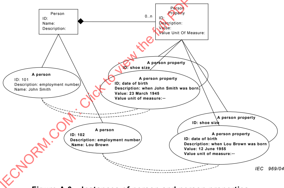
Figure A.6 – Instances of person and person properties
