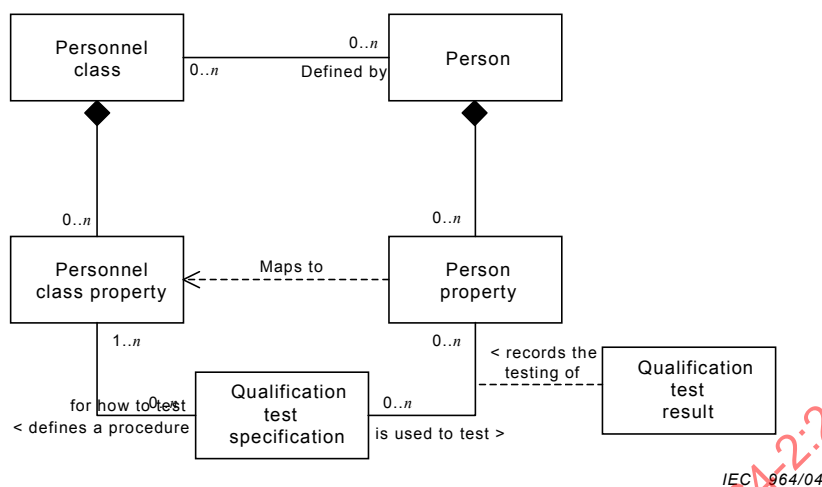
Figure A.1 – Personnel model
