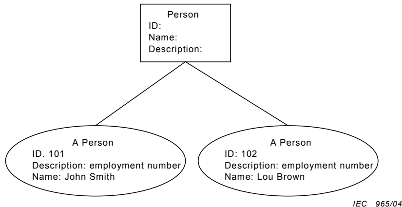
Figure A.2 – Instances of a person class
