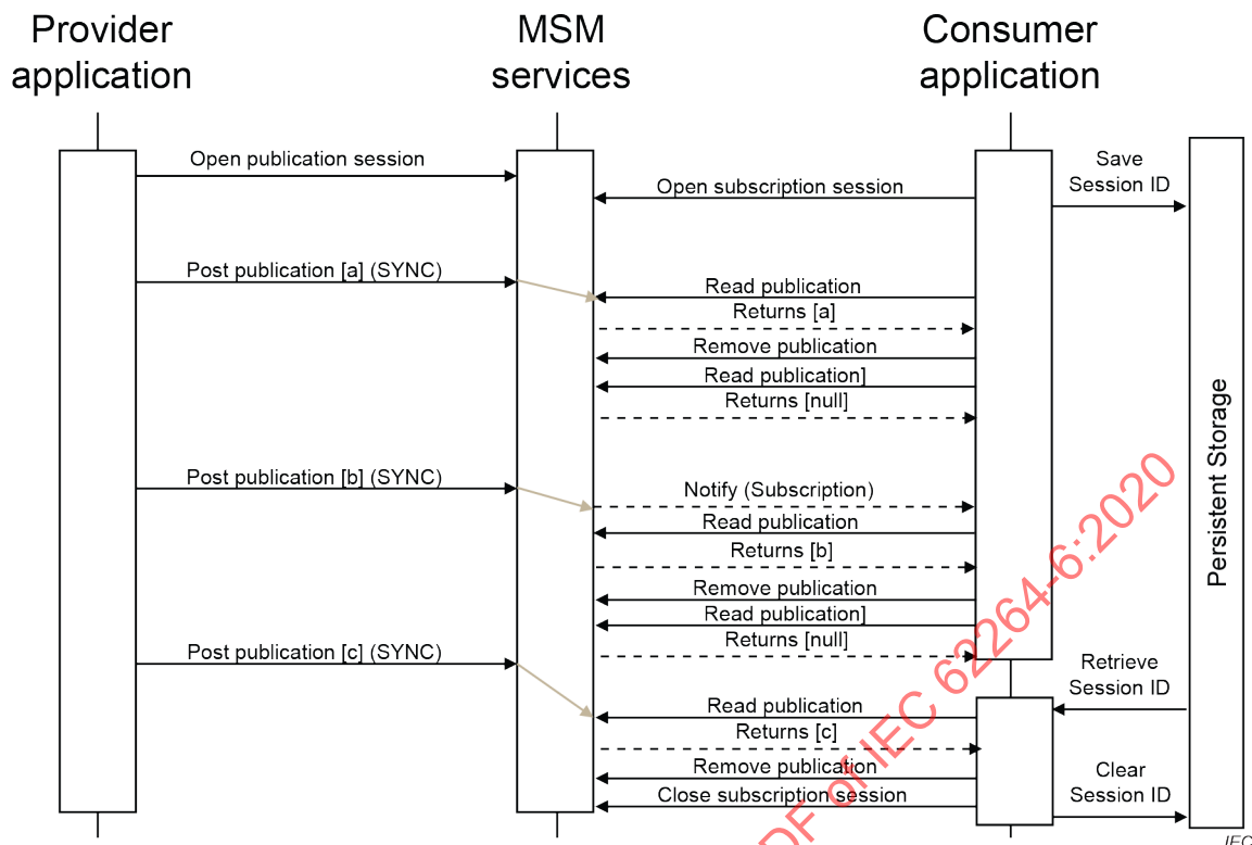
Figure 12 – Publication scenario with multiple messages
