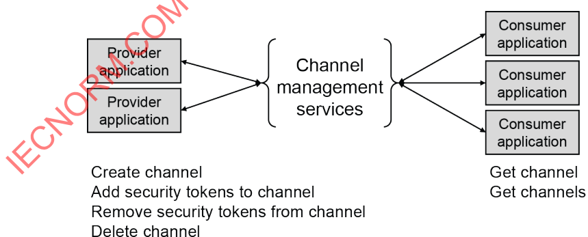
Figure 5 – Channel management services
