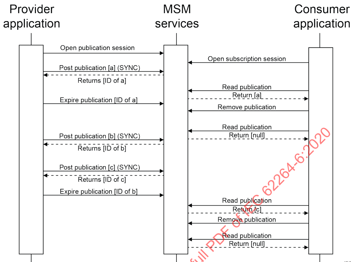
Figure 15 – Publication with expired publications
