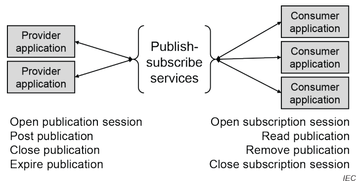
Figure 6 – Publication channel services
