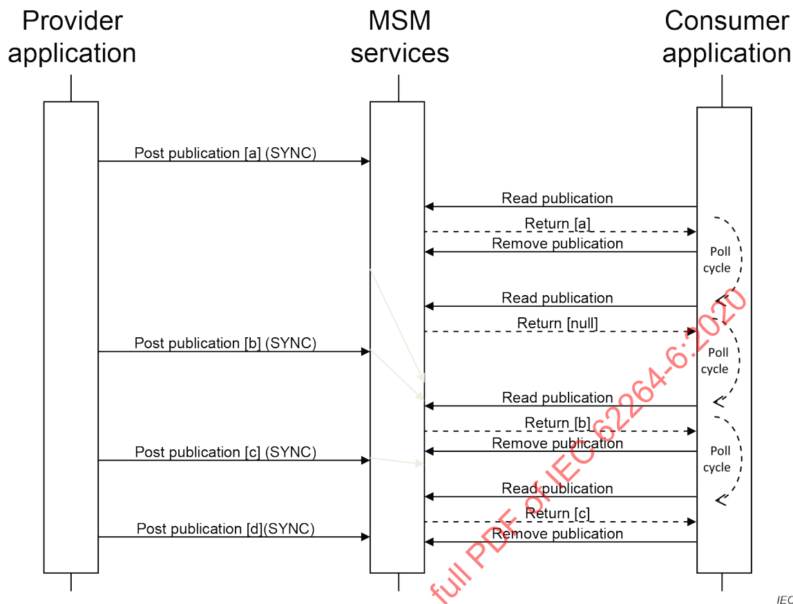
Figure 13 – Publication without notification
