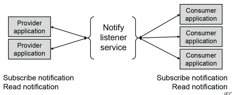
Figure 8 – Notify listener service
