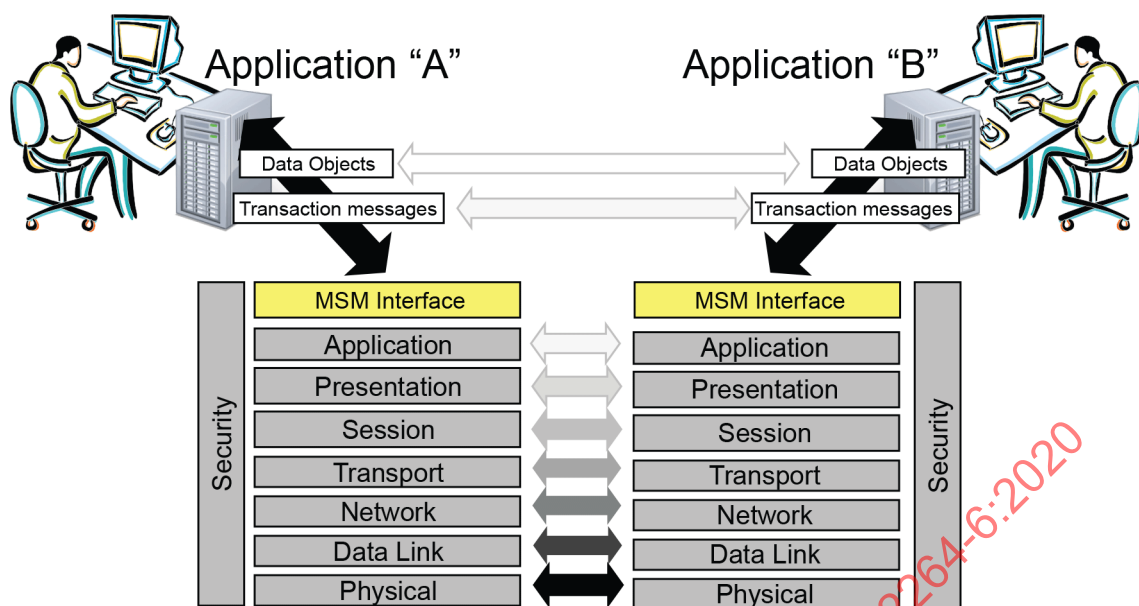
Figure 3 – Positioning and role of MSM
