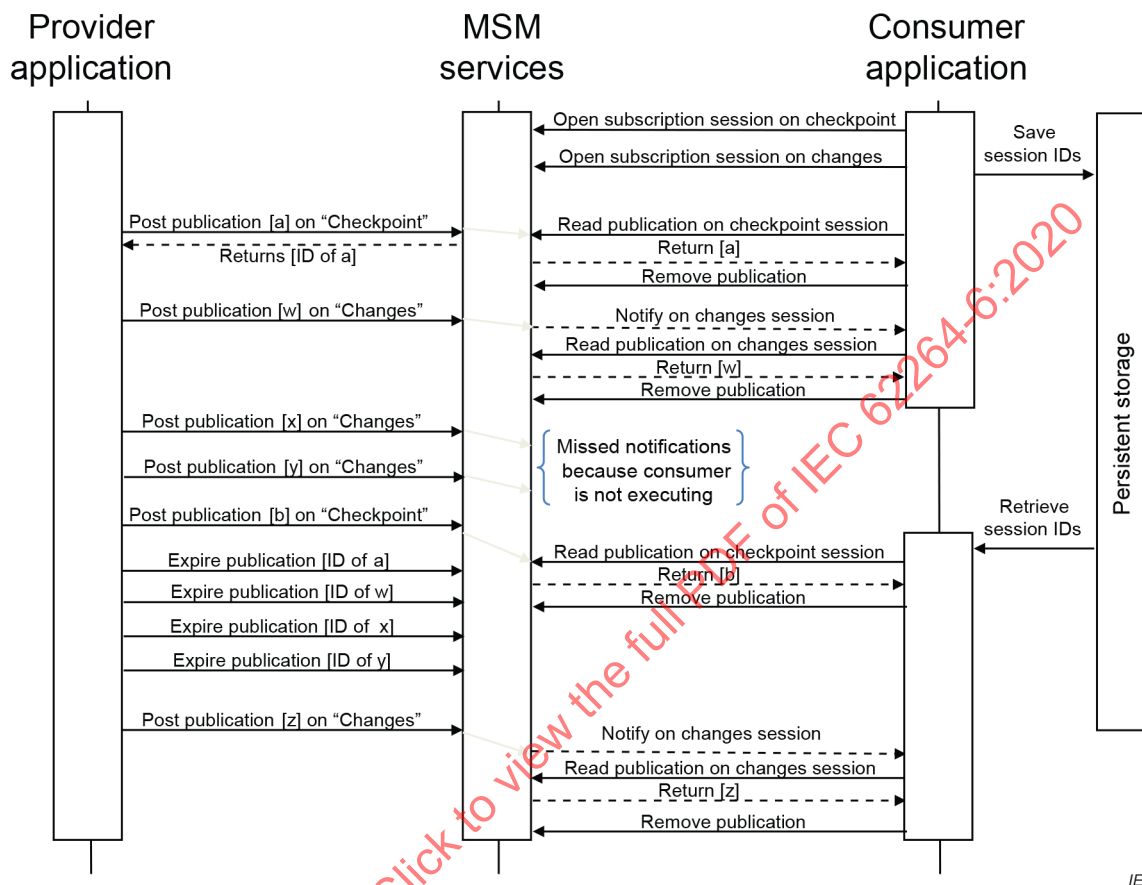
Figure 9 – Changes and checkpoint channel example
