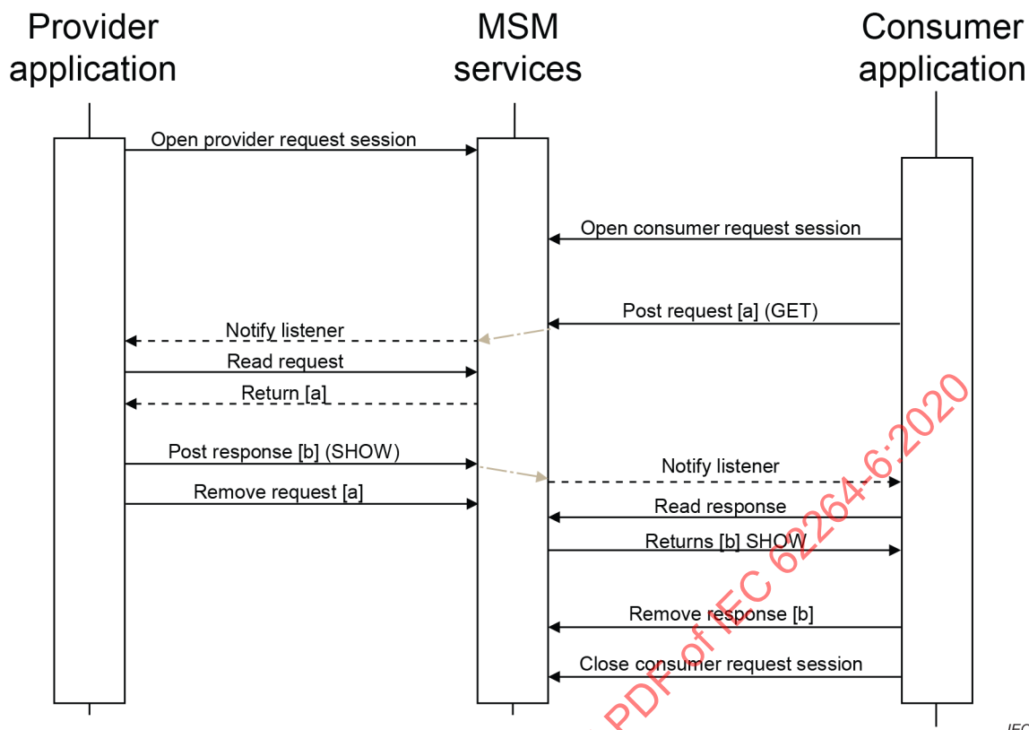
Figure 16 – GET/SHOW request service scenario
