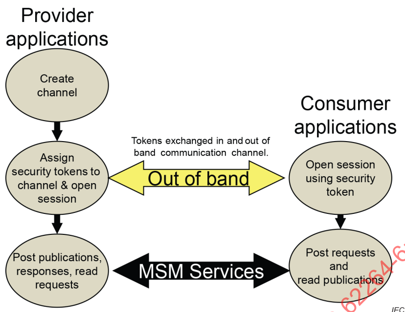
Figure 10 – Security of channels
