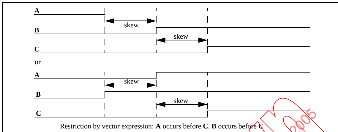
Figure 33—Illustration of SKEW
