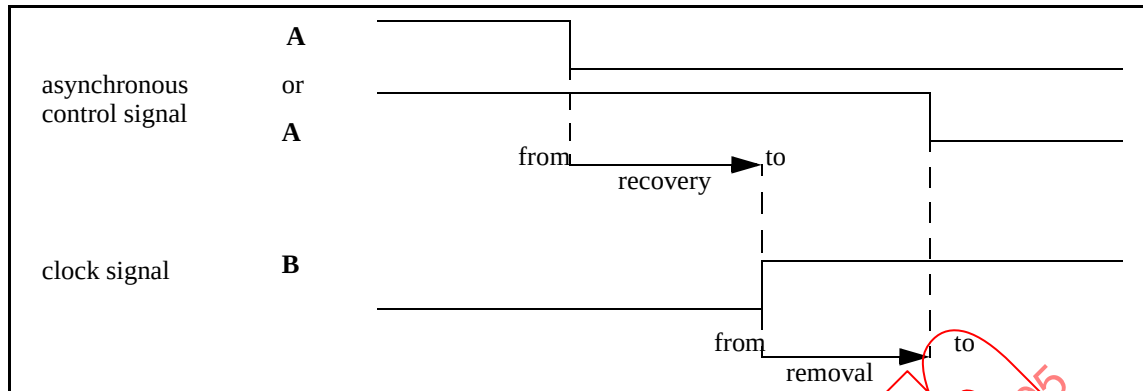
Figure 28—RECOVERY and REMOVAL
