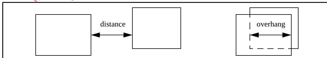
Figure 43—Illustration of DISTANCE versus OVERHANG
