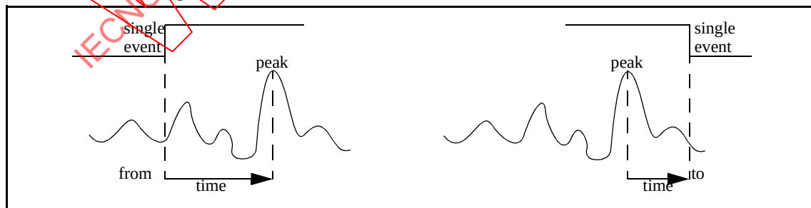
Figure 38—Illustration of peak measurement with FROM or TO statement
