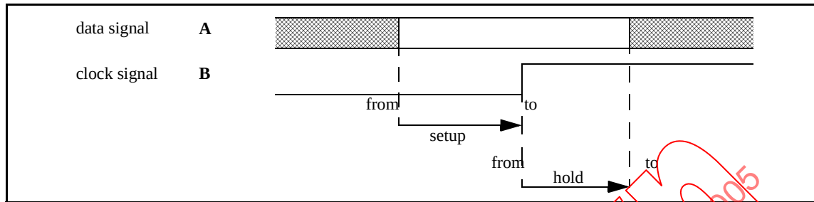
Figure 27—Illustration of SETUP and HOLD
