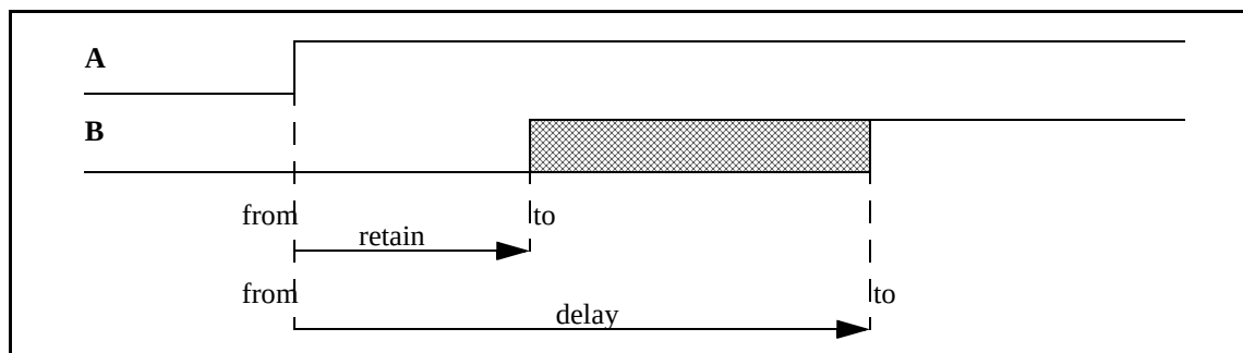
Figure 25—Illustration of RETAIN and DELAY
