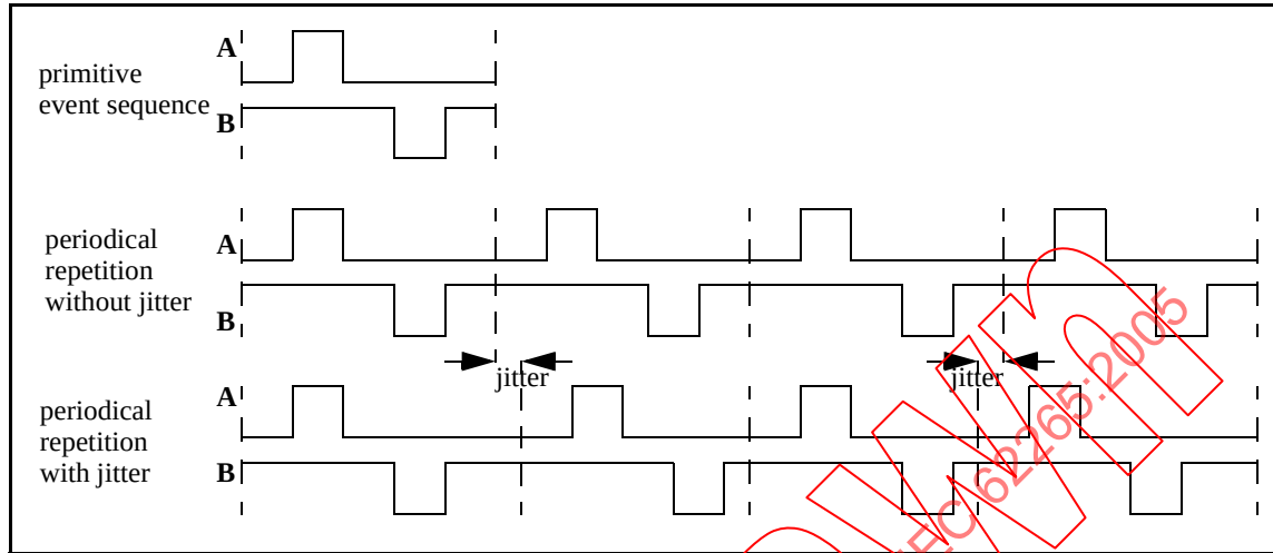
Figure 32—Illustration of JITTER
