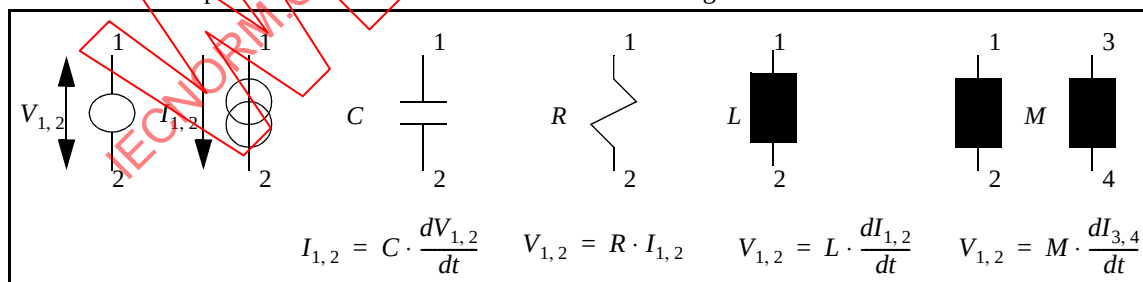
Figure 39—Electrical components and their terminals
