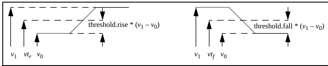
Figure 34—THRESHOLD measurement definition
