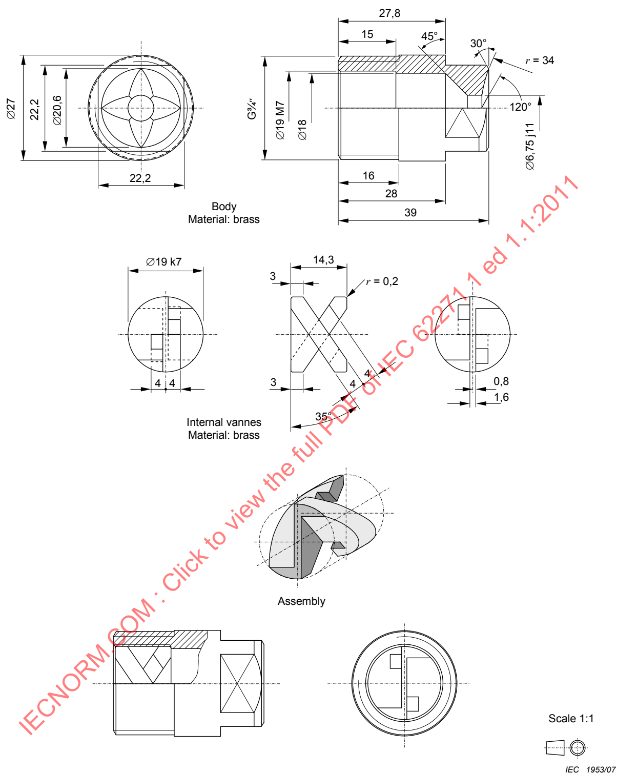
Figure C.2 – Nozzle for weatherproofing test
