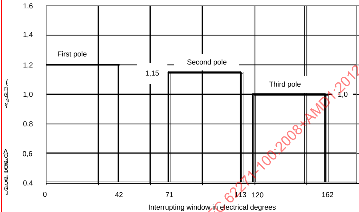
Figure 58 – Graphical representation of the interrupting window and the voltage factor k_p , determining the TRV of the individual pole, for systems with a first-pole-to-clear factor of 1,2
