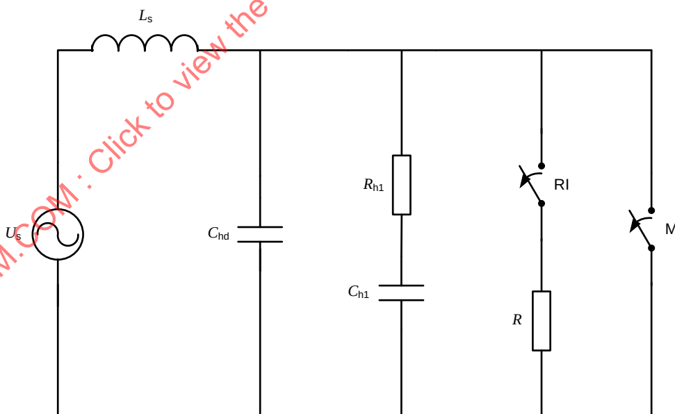
Figure R.2 – Test circuit for test duties T60 and T100
