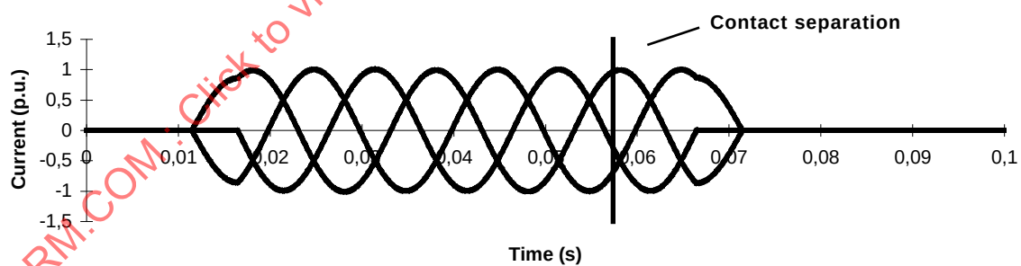
Figure 29 – Example of a graphical representation of the three valid symmetrical breaking operations for three-phase tests in a non-effectively earthed neutral system (first-pole-to-clear factor 1,5)
