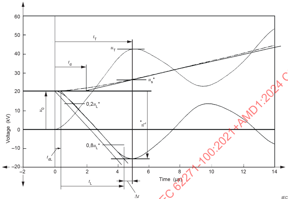
Figure A.1 – Typical graph of line and source side TRV parameters – Line side and source side with time delay
