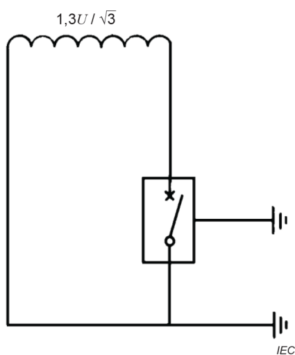
Figure 20a – Preferred circuit
