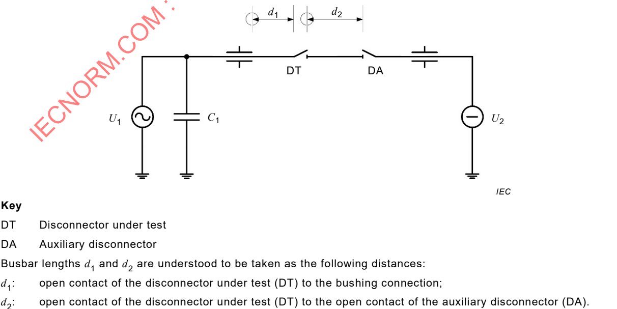
Figure 14 – Test circuit for test duty 1
