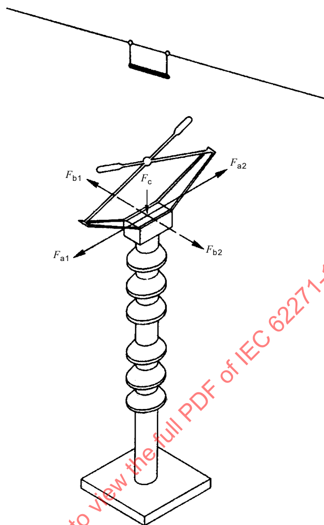
Figure 11 – Example of the application of rated static mechanical terminal loads to a (divided support) pantograph disconnector (or earthing switch)
