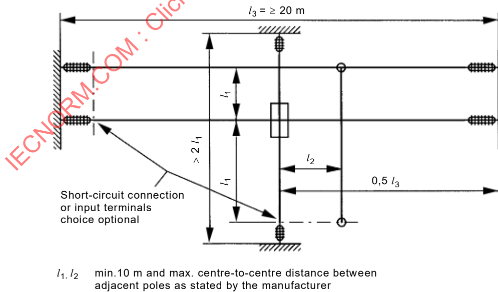
b) Test arrangement for disconnectors of U_r > 550 \text{ kV}
