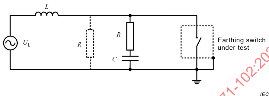
Figure 15 – Test circuit for electromagnetically induced current switching tests
