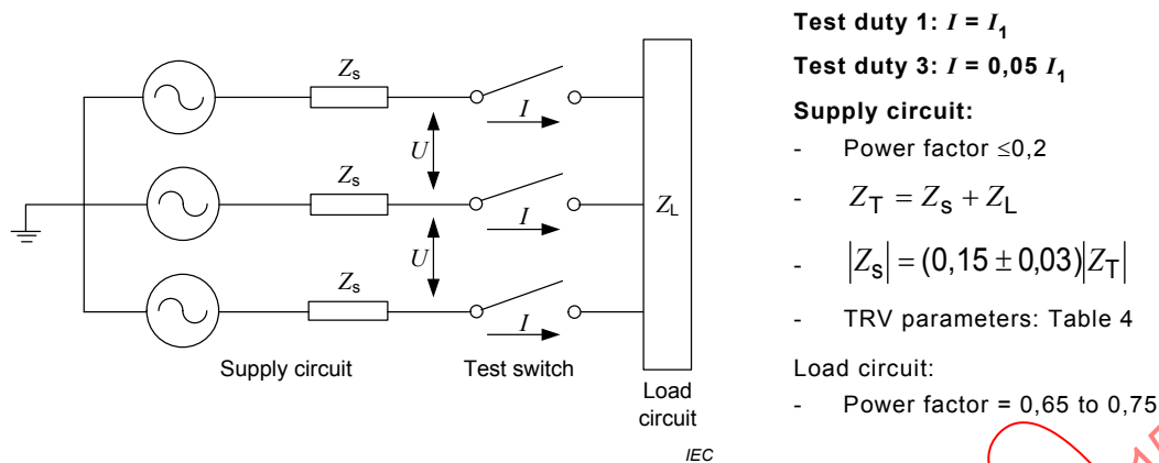
Figure 3a – General circuit
