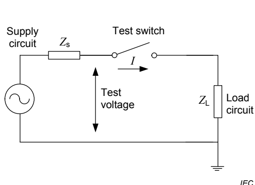
Figure 1 – Single-phase test circuit for mainly active load current switching for test duties 1 and 3
