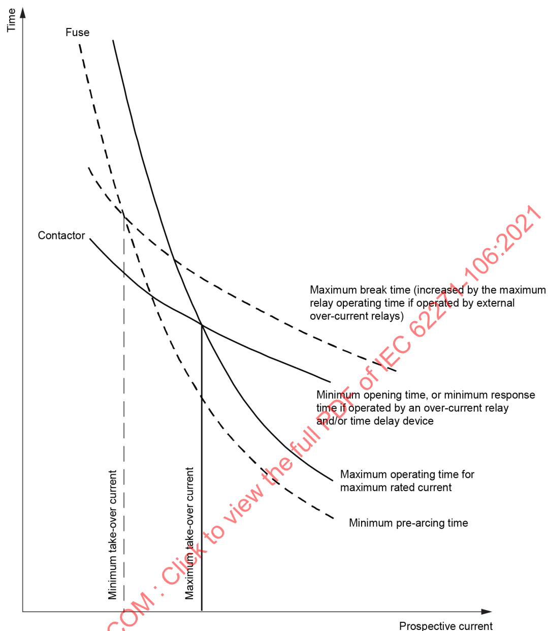
Figure 9 – Characteristics for determining take-over current
