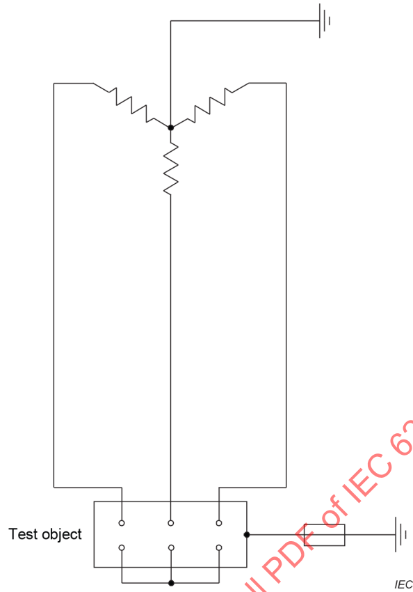
Figure 6 – Test duties A and B – alternative earth point
