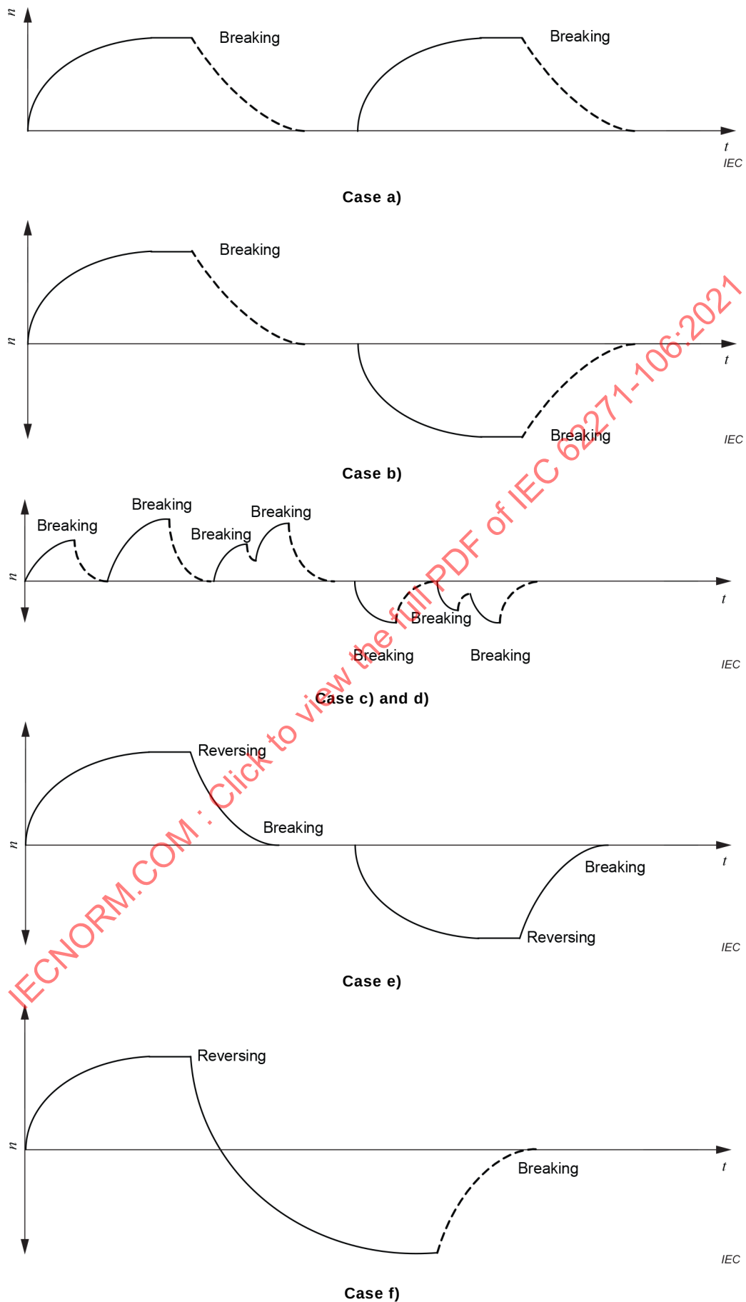
Figure 1 – Examples of speed/time curves
