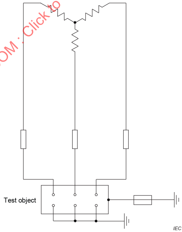
Figure 7 – Test duty C – preferred earth point
