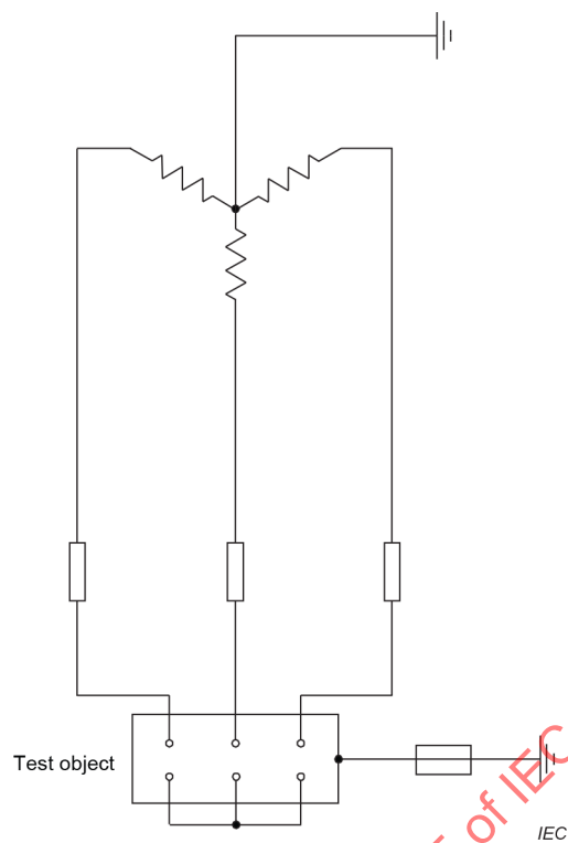
Figure 8 – Test duty C – alternative earth point
