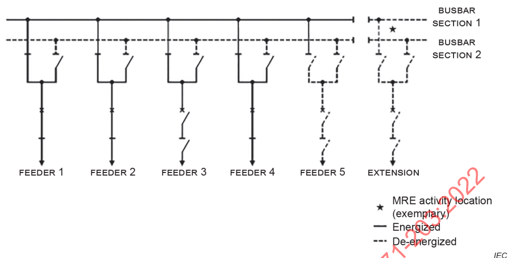
Figure F.5 – MRE11 (e.g. extension of switchgear with a feeder bay)
