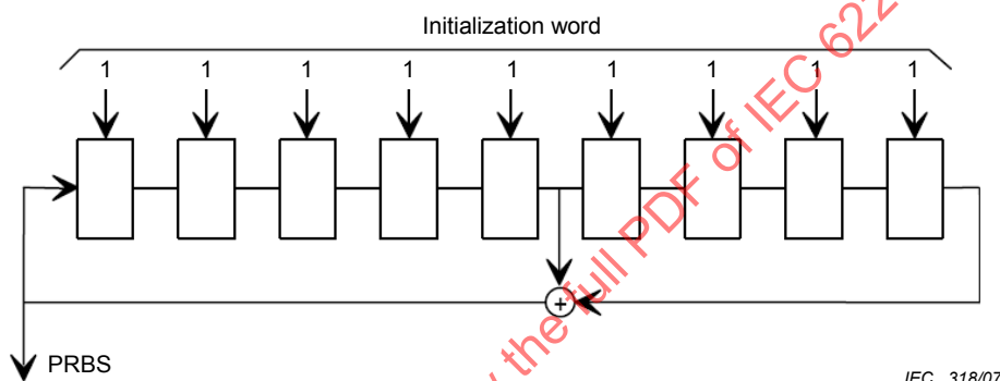
Figure 3 – PRBS generator
