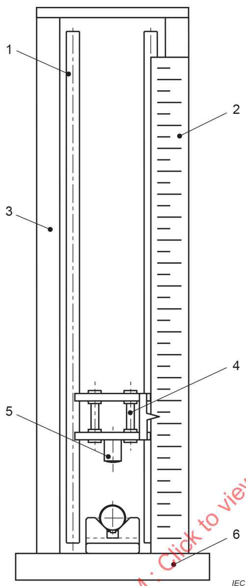
Figure 4 a) – Test apparatus assembly
