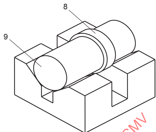
Figure 4 c) – Position of tie strap
