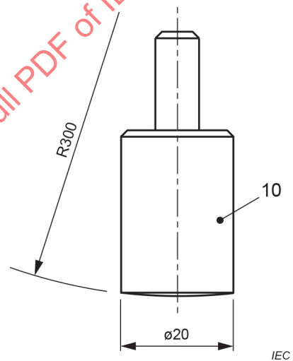
Figure 4 d) – Hammer details
