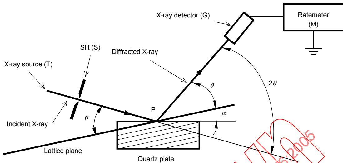
Figure 9 – Measurement method by X-ray
