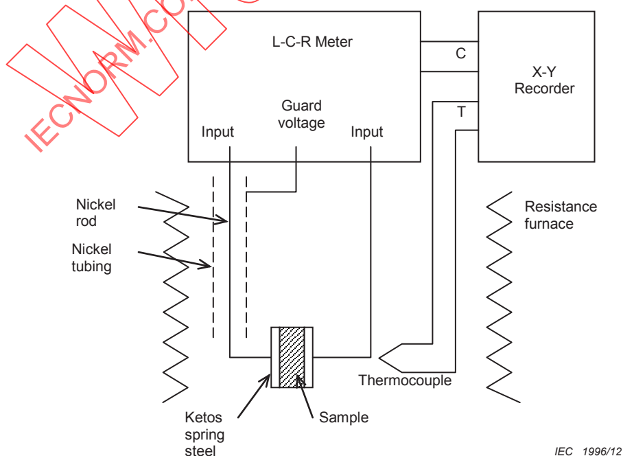
Figure 7 – Schematic of a dielectric constant measurement system
