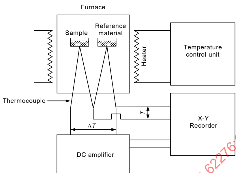
Figure 7 – Schematic of a DTA system
