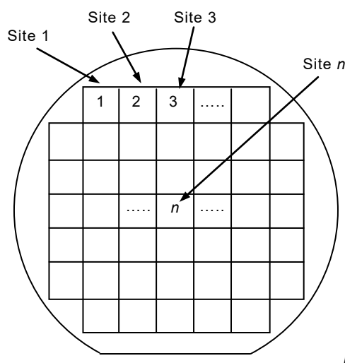
Figure 5 – Example of site distribution for LTV measurement
