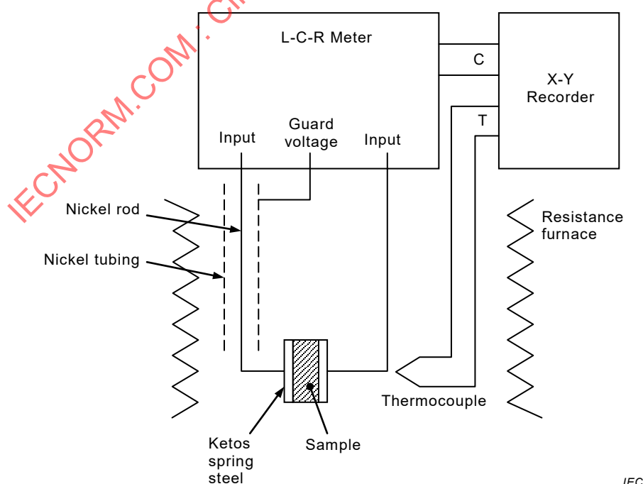
Figure 8 – Schematic of a dielectric constant measurement system
