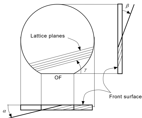
Figure 11 – Relationship between cut angle and lattice planes
