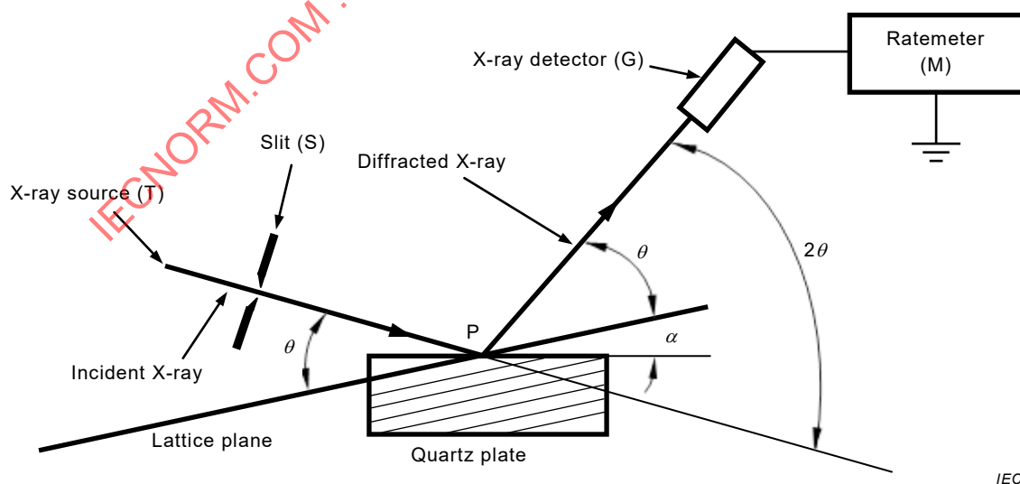
Figure 10 – Measurement method by X-ray
