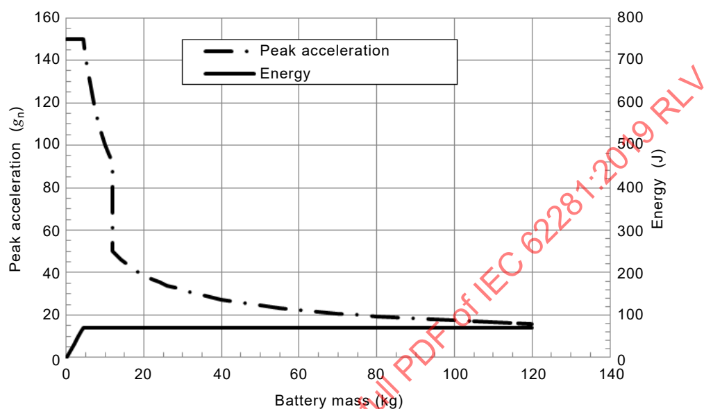
Figure A.2 – Half sine shock for batteries (constant energy)
