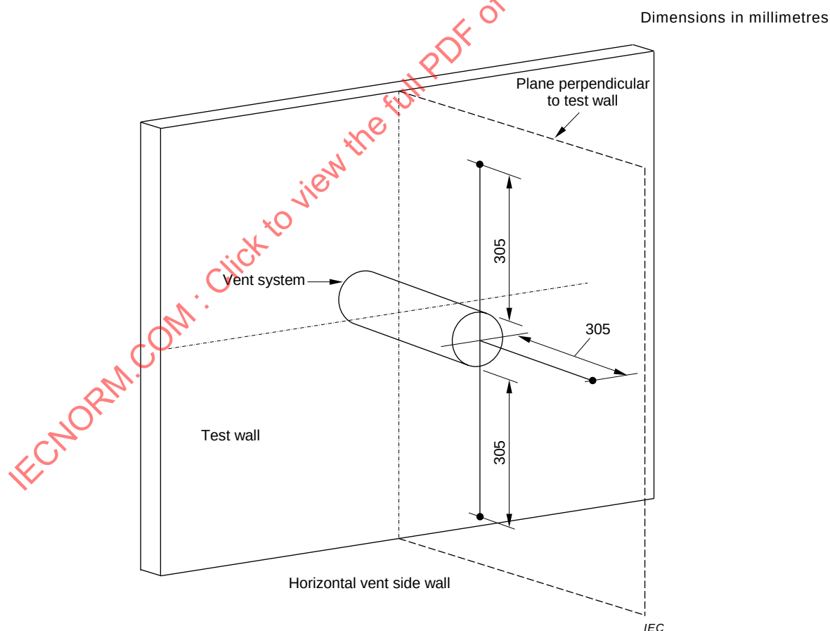
Figure 4 – Vent test wall
