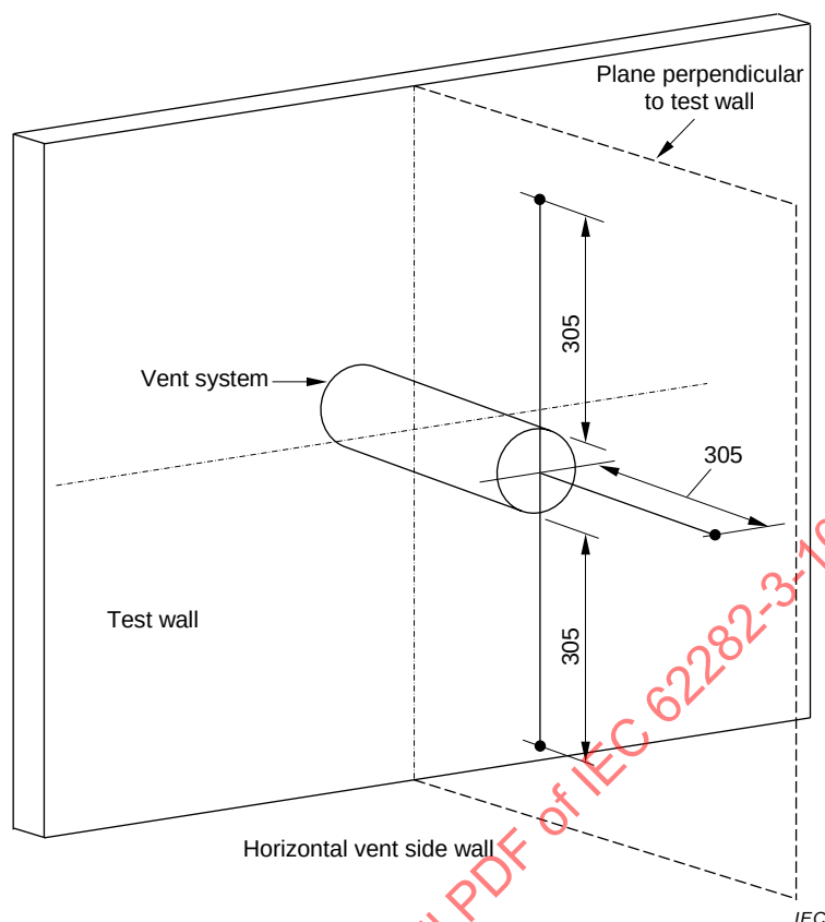
Figure 4 – Vent test wall
