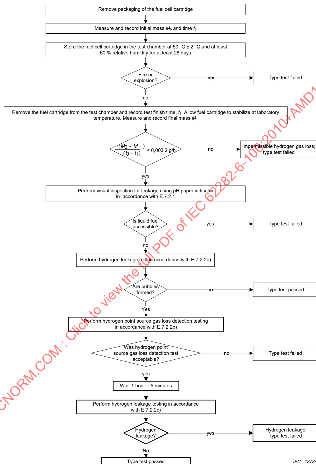
Figure E.9 – Fuel cartridge hydrogen leakage and mass loss test flowchart for long-term storage test – Replaces Figure 9
