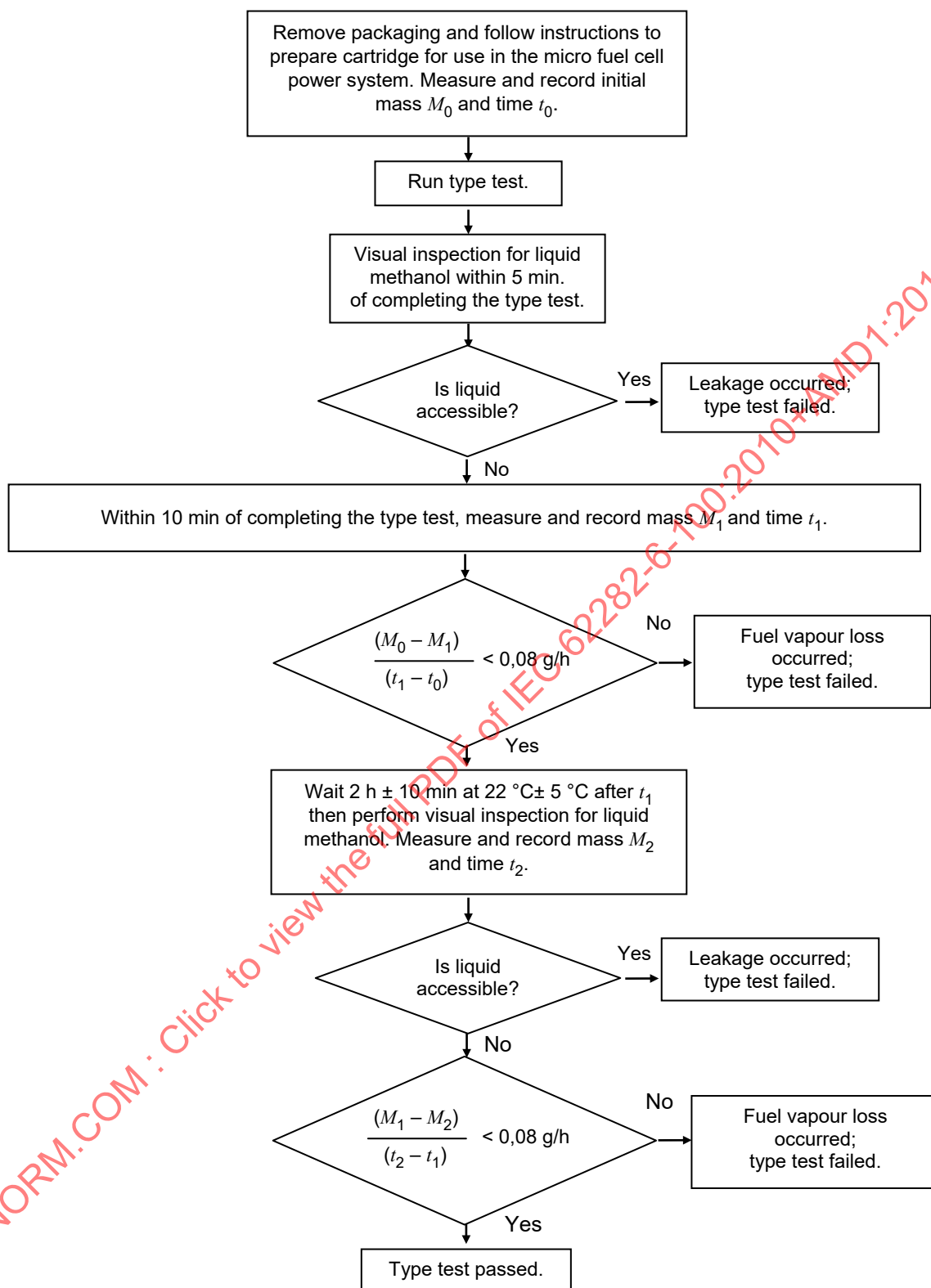
Figure 2 – Fuel cartridge leakage and mass loss test flow chart for pressure differential, vibration, drop, and compressive loading tests
