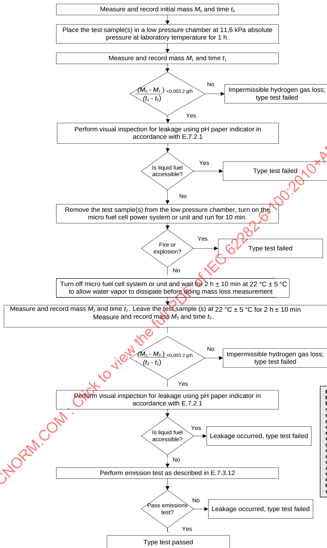
Figure E.7 – Micro fuel cell power system or micro fuel cell power unit leakage and mass hydrogen gas loss test flow chart for 11,6 kPa low external pressure test – Replaces Figure 7
