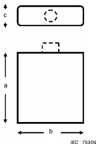
Figure 55 – Prismatic cartridge
