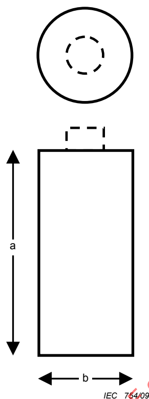
Figure 56 – Cylindrical cartridge
