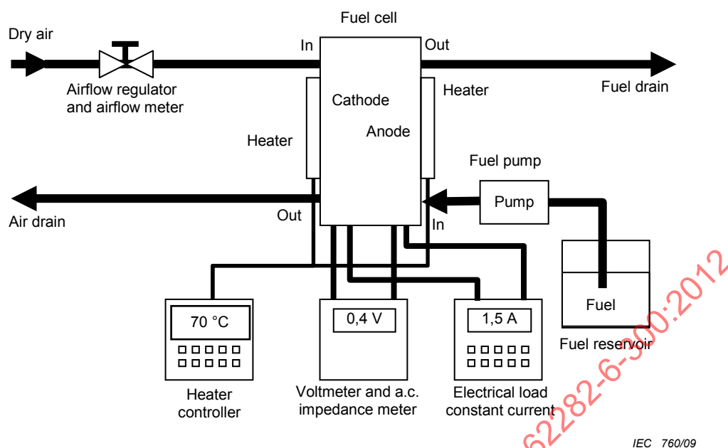
Figure 62 – Test apparatus
