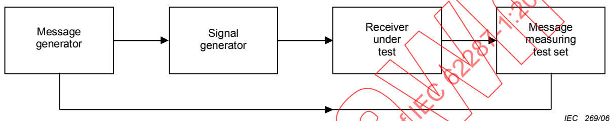
Figure 12 – Measurement arrangement
