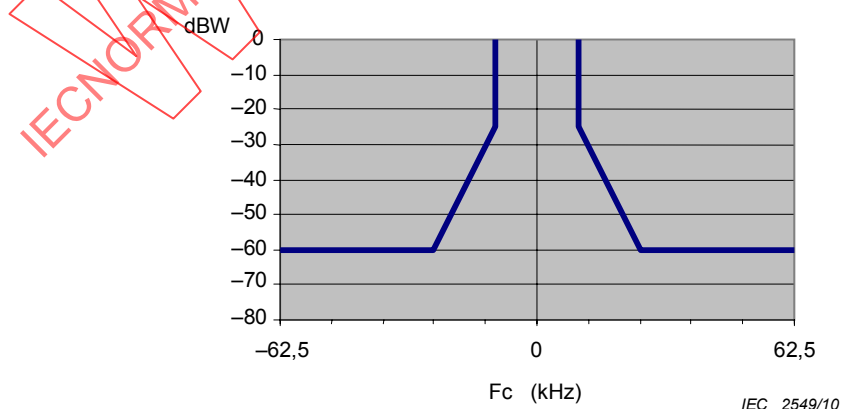
Figure 10 – Emission mask
