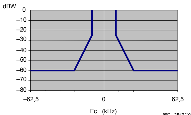
Figure 10 – Emission mask
