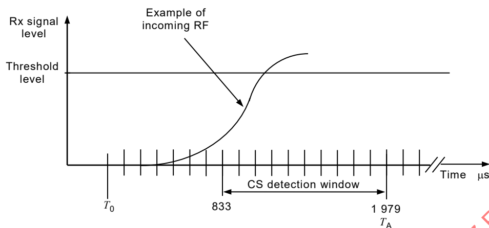
Figure 2 – Carrier-sense timing
