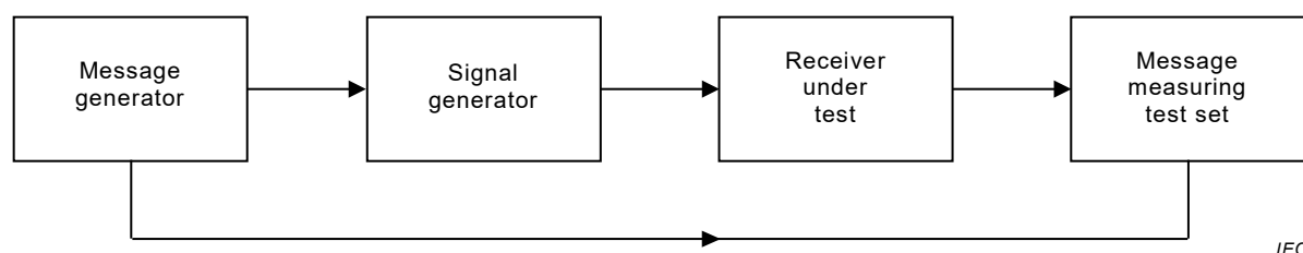
Figure 12 – Measurement arrangement
