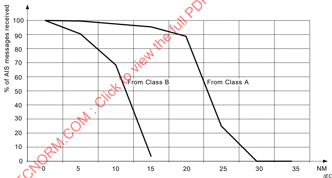
Figure A.3 – Reception of messages by Class B AIS
