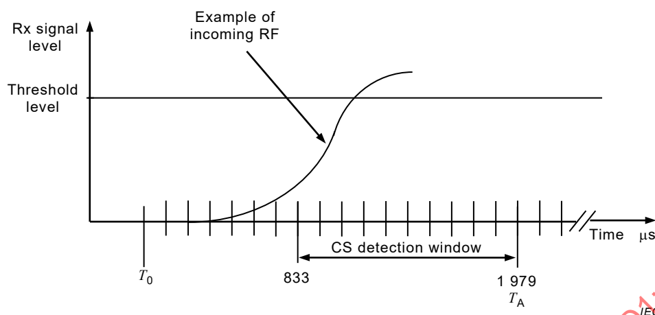
Figure 2 – Carrier-sense timing
