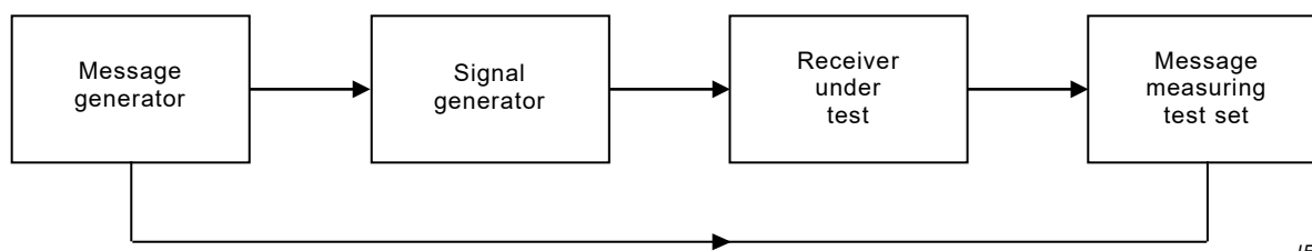
Figure 12 – Measurement arrangement
