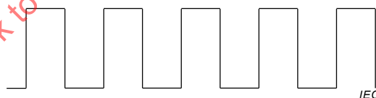
Figure 5a – Unmodified bit pattern
