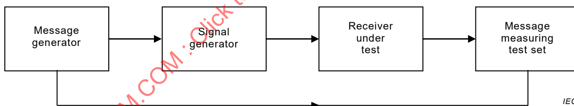
Figure 7 – Measurement arrangement
