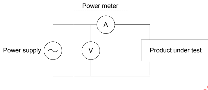
Figure B.1 – Connection arrangement for products powered directly from an a.c. power supply for lower power loads
