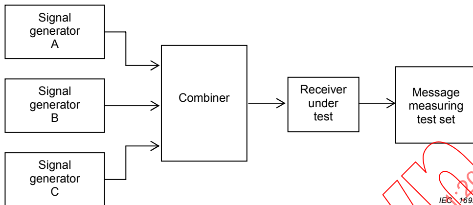
Figure 19 – Measurement arrangement for inter-modulation
