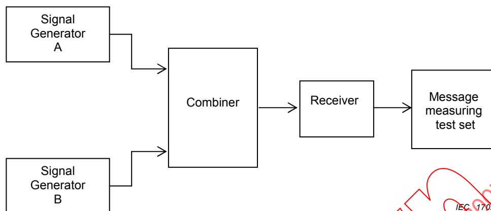
Figure 20 – Measurement arrangement for blocking or de-sensitisation
