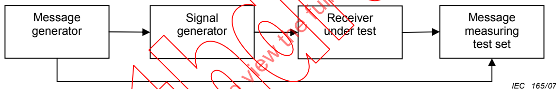
Figure 15 – Measurement arrangement
