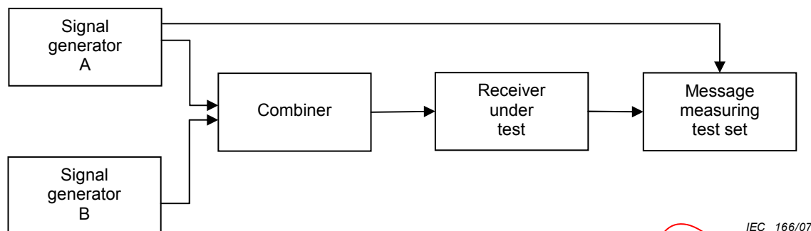
Figure 16 – Measurement arrangement
