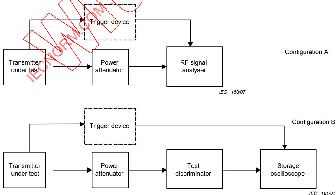
Figure 11 – Measurement arrangement for modulation accuracy
