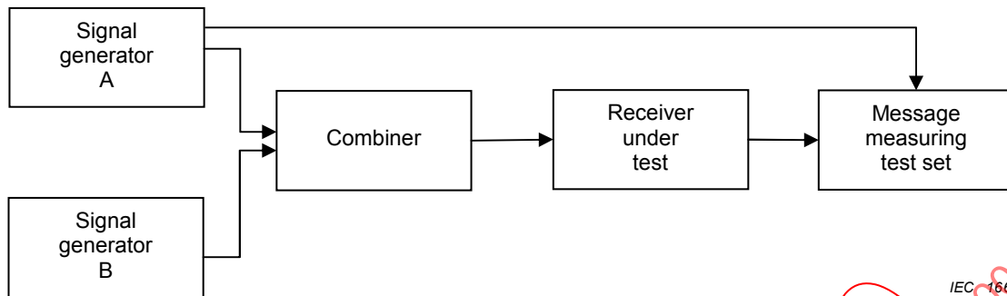
Figure 16 – Measurement arrangement
