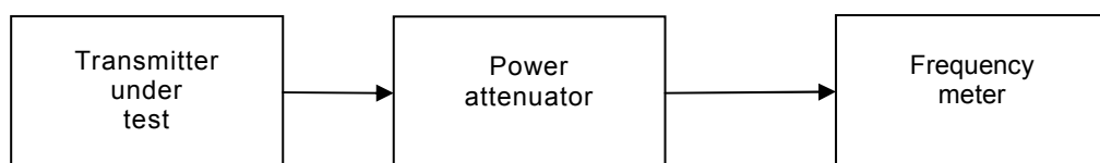
Figure 7 – Measurement arrangement
