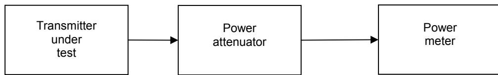
Figure 8 – Measurement arrangement
