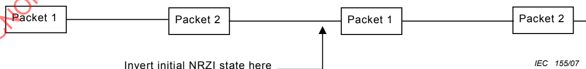
Figure 6 – Format for repeating four-packet cluster
